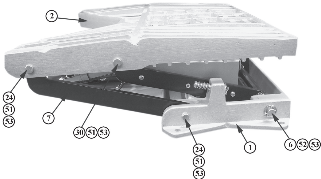
FIGURE 10 - SIDE VIEW
