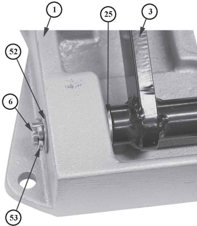
FIGURE 5 - TORQUE TUBE
