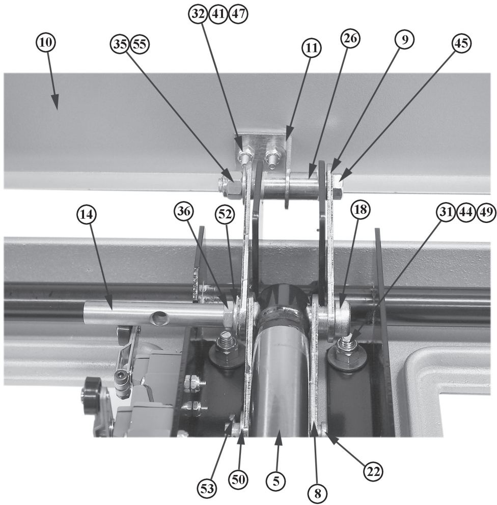
FIGURE 9 - KICK PLATE ATTACHMENT
