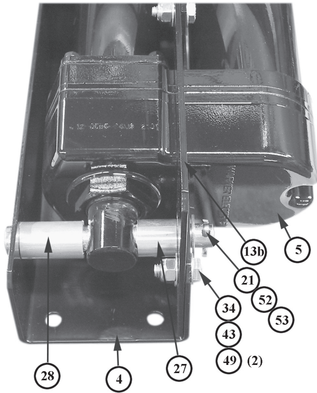
FIGURE 4 - ACTUATOR
