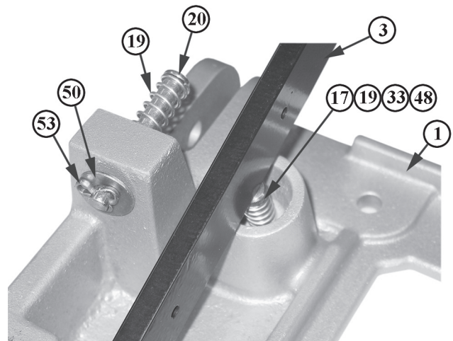
FIGURE 11 - SPRINGS
