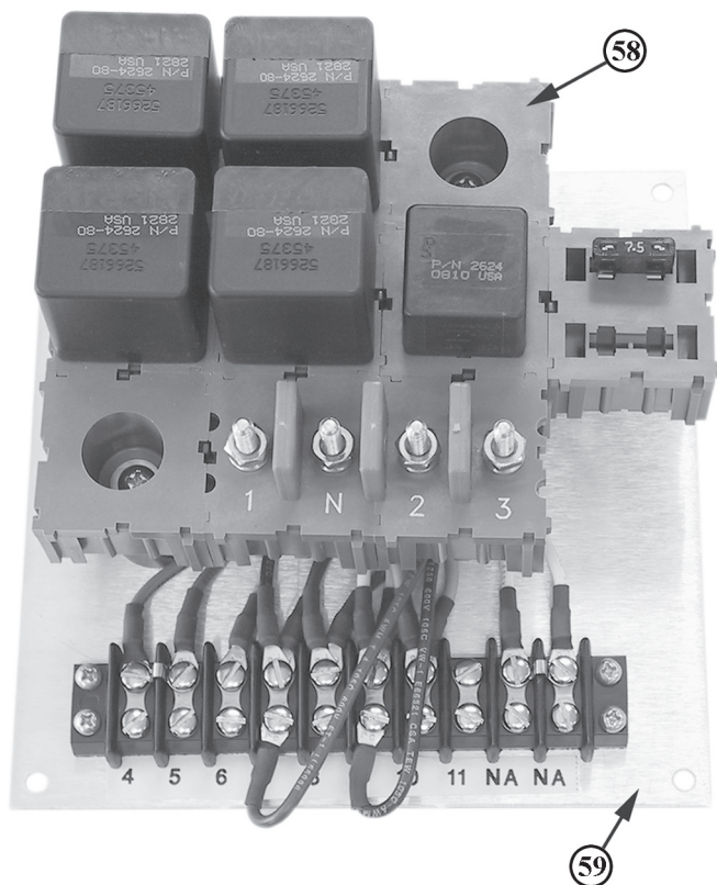
FIGURE 3 - ELECTRICAL PANEL
