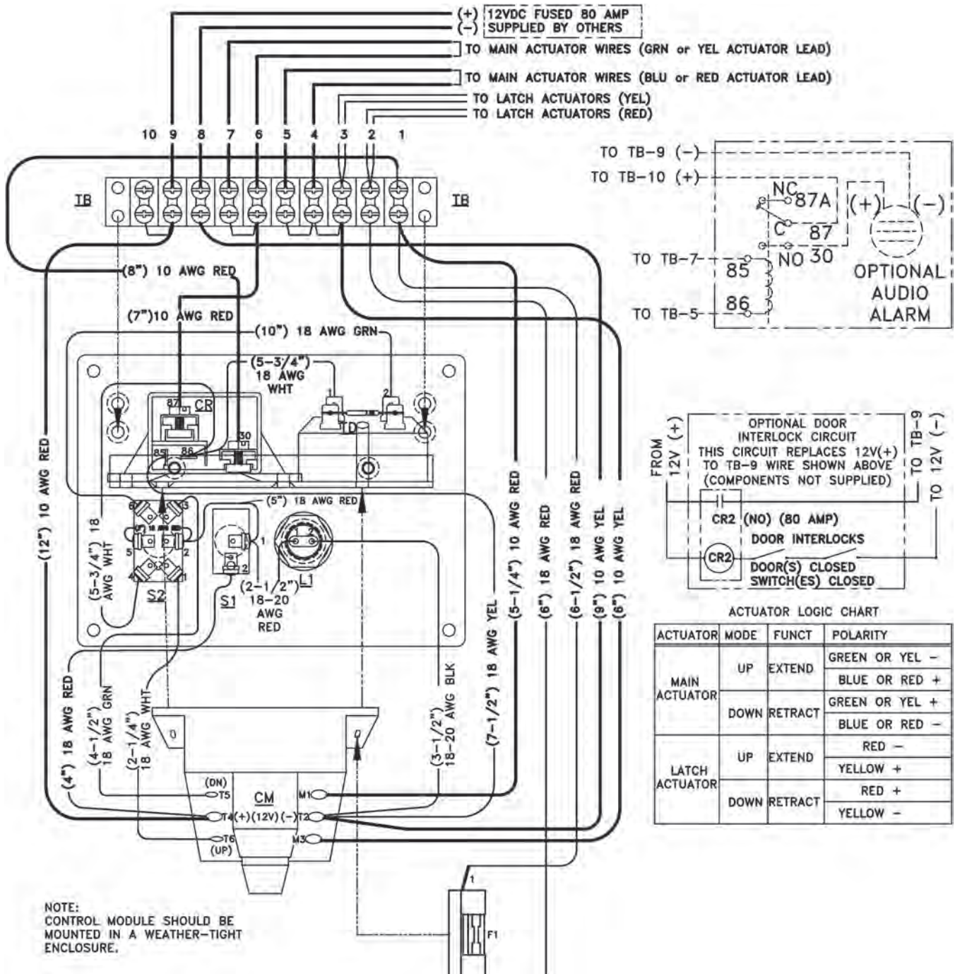
FIGURE 20. ELECTRICAL SYSTEM WHEN USING ELECTRIC LOCKS
