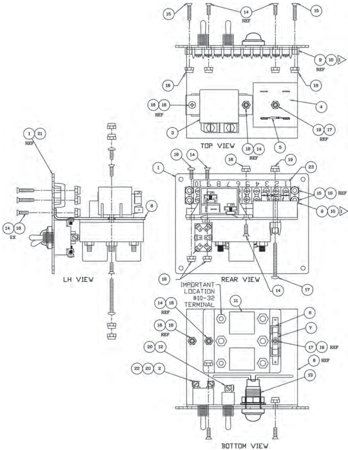
FIGURE 21. CONTROL PANEL ASSEMBLY
