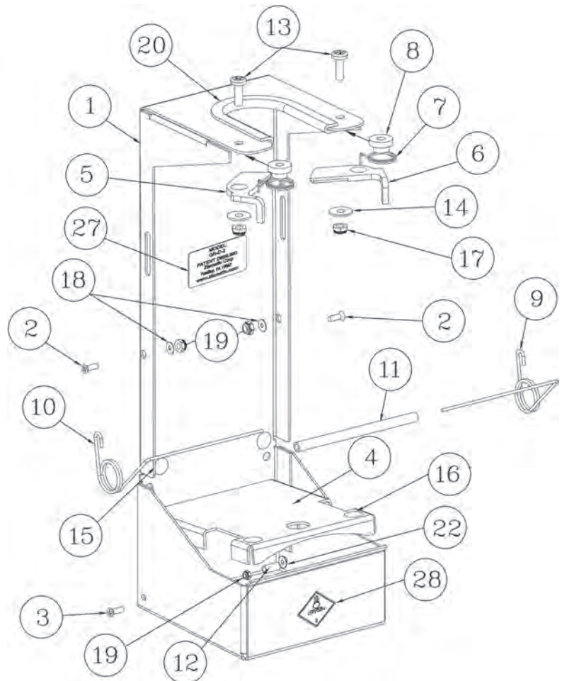
EXPLODED VIEW
