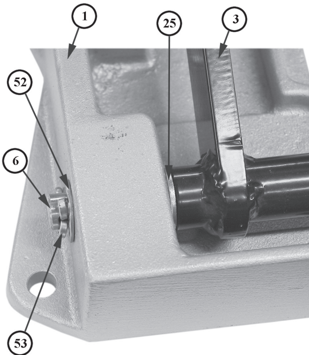
FIGURE 4 - TORQUE TUBE
